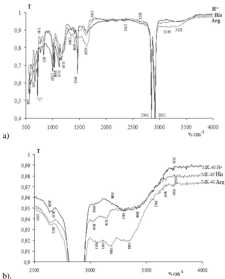
Fig. 1. IR-spectra of membrane MK-40 in arginine, histidine and \text{H}^+ -forms. a) 500-4000 \text{cm}^{-1} , b) 2500-4000 \text{cm}^{-1}
