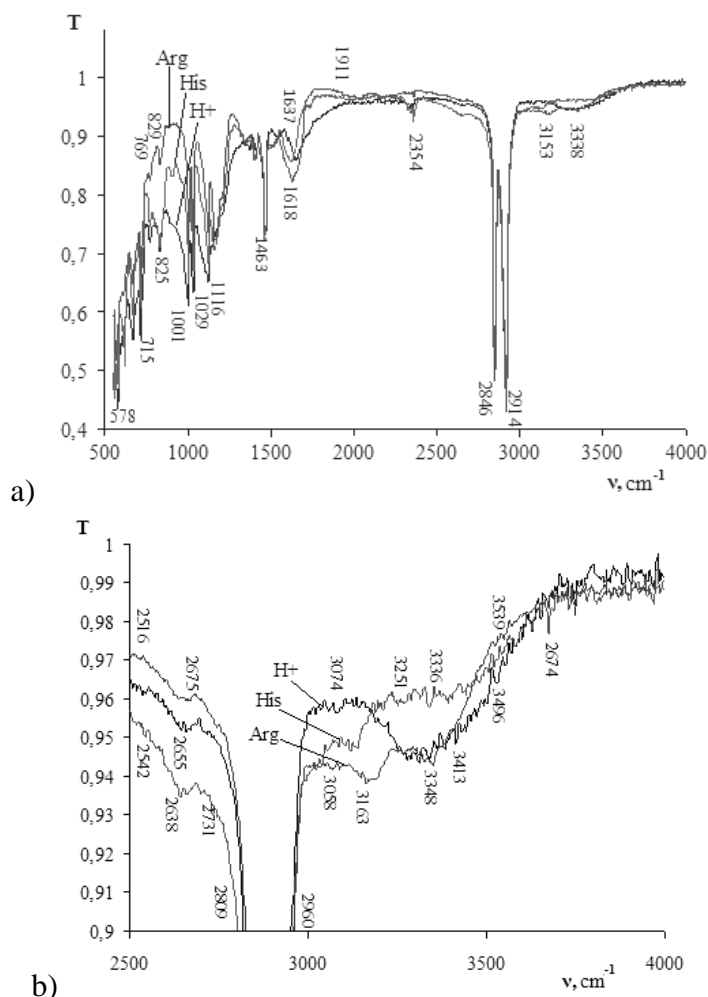
Fig. 2. IR-spectra of FTCEM-E membrane in arginine, histidine and \text{H}^+ -forms.
